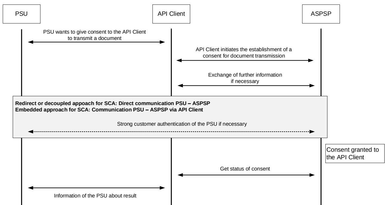
Figure 3: API Service: Establish consent for document transmission
