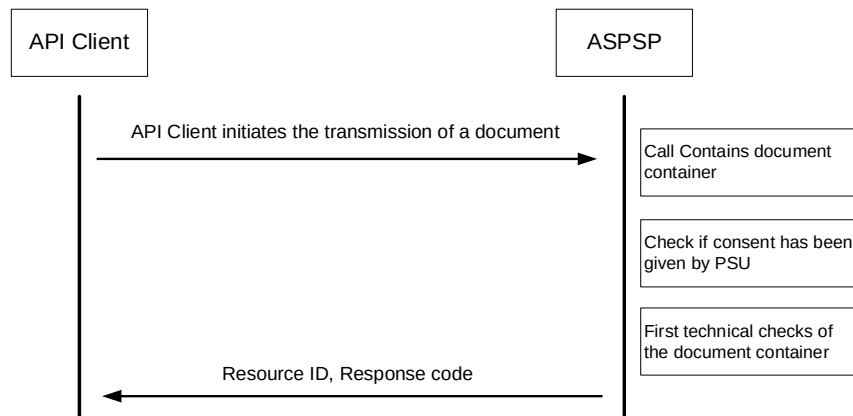
Figure 6: API Service: Document transmission
