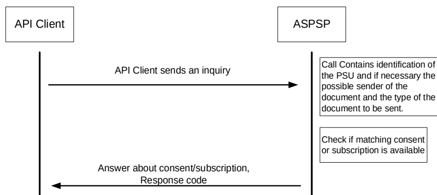
Figure 4: API Service: Reachability check
