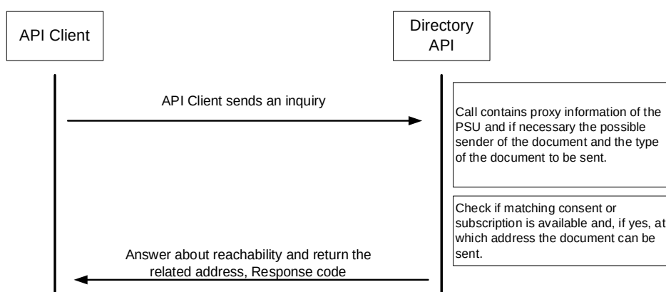
Figure 5: API Service: Lookup Function
