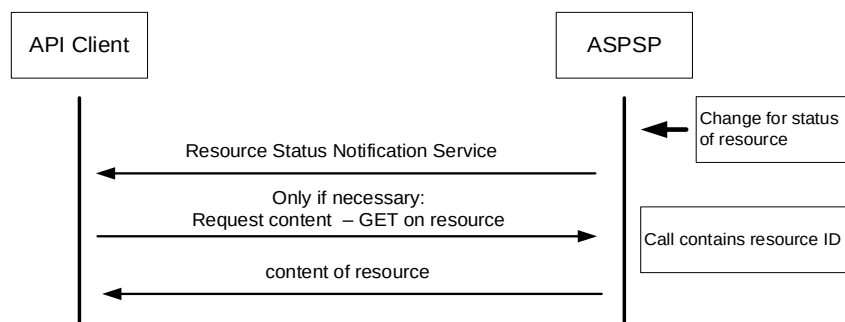
Figure 9: API Service: Document Status with Resource Status Notification Service
