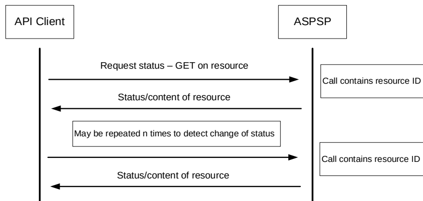
Figure 8: API Service: Document Status with polling
