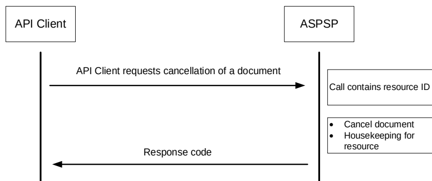
Figure 7: API Service: Document cancellation
